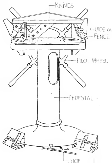
TRIANGULAR ATTACHMENT— FIG. 207. TRIMMER.
